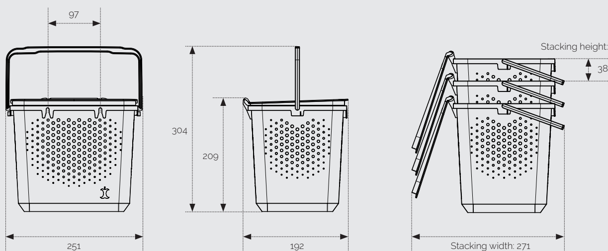
General dimensions
